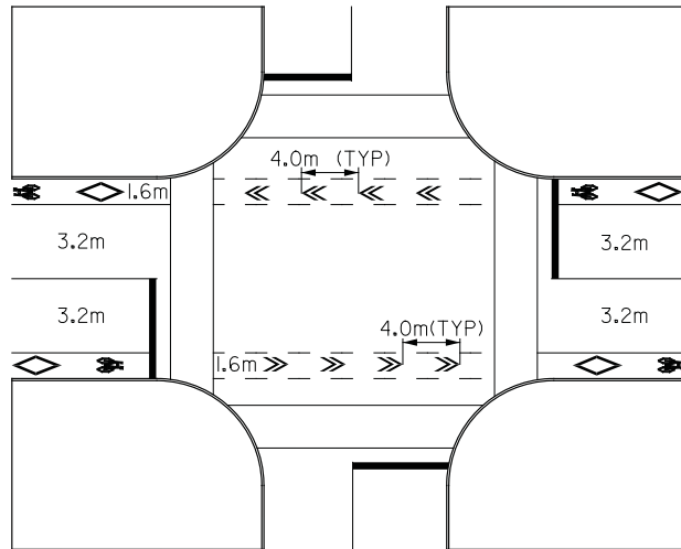
Intersection treatment along a bike lane.
