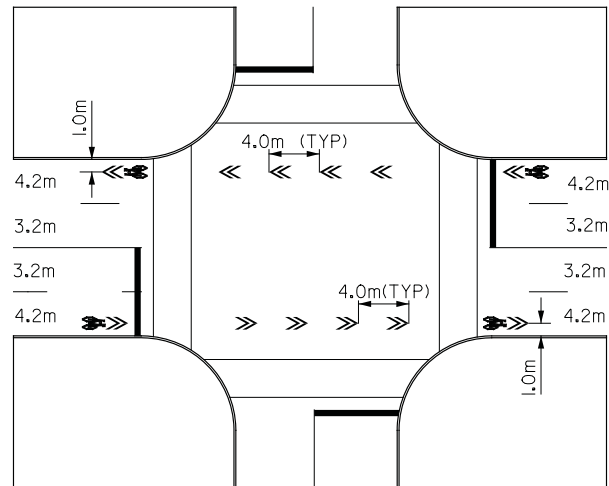
Intersection treatment along a sharrow route.
