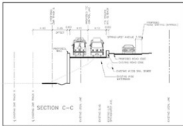
CROSS-SECTIONS
