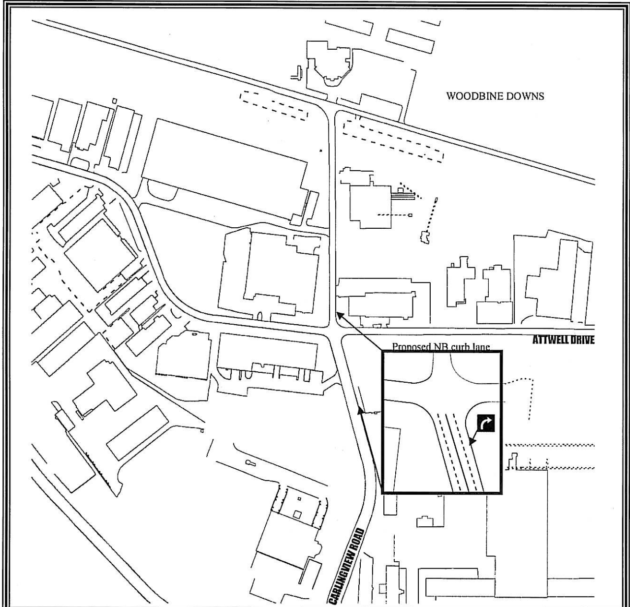
Proposed Exclusive Right Turn Lane Northbound on Carlingview Road at Attwell Drive
