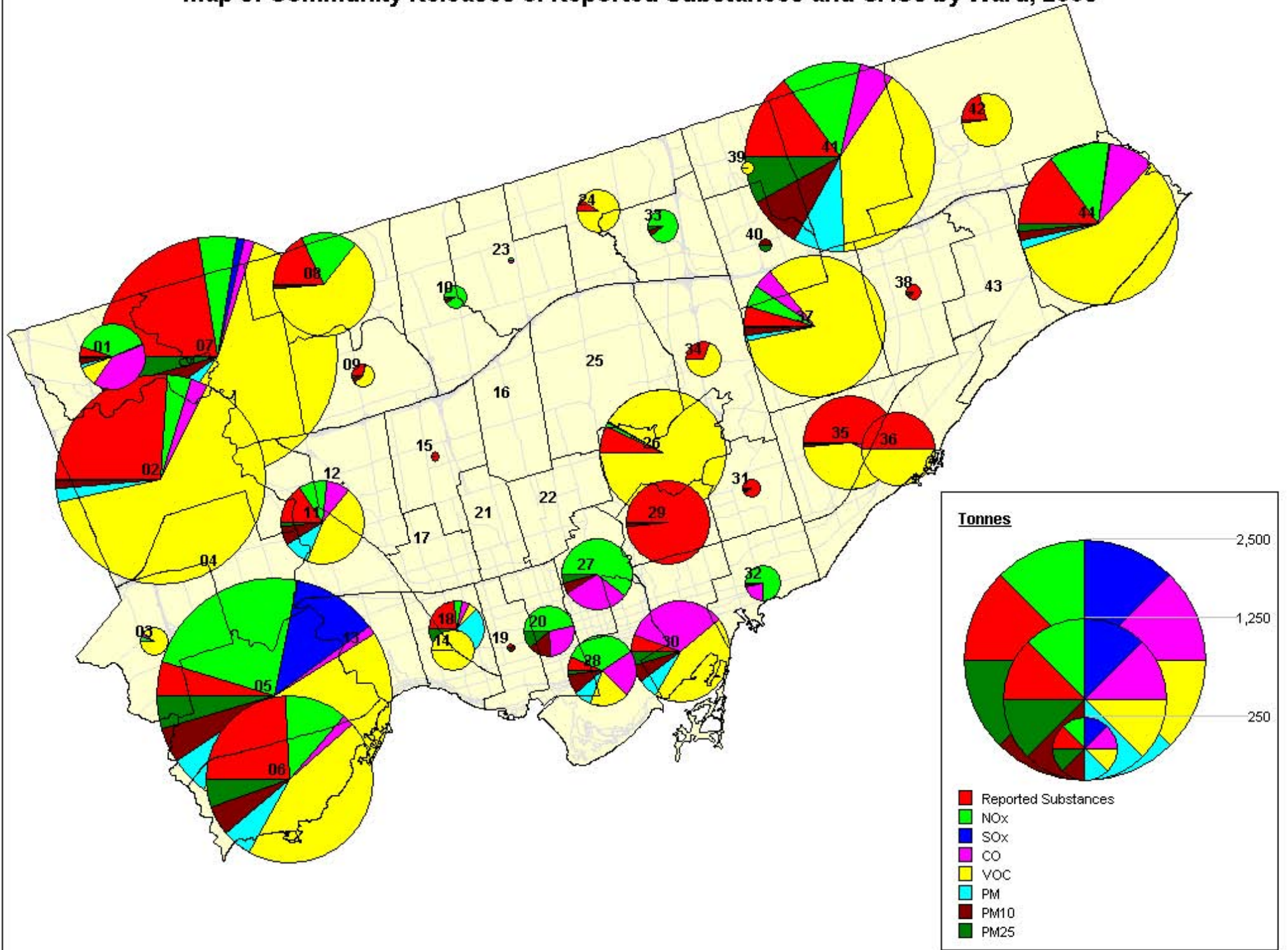
Map 3: Community Releases of Reported Substances and CACs by Ward, 2005
