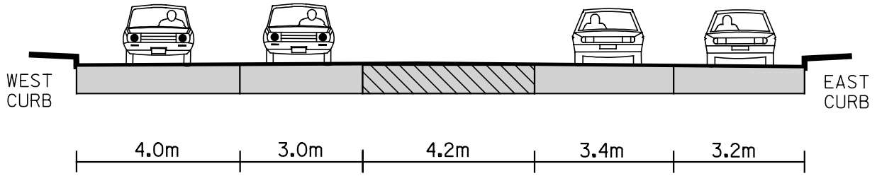
EXISTING CROSS SECTION B - B PAVEMENT WIDTH VARIES
