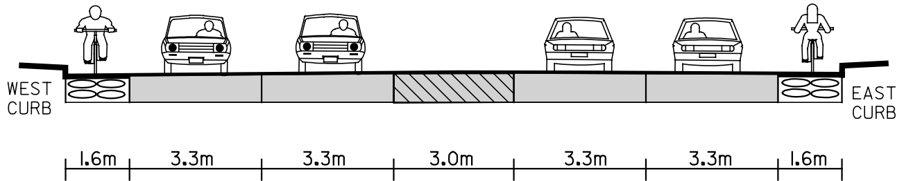
PROPOSED CROSS SECTION B - B PAVEMENT WIDTH: 19.4m
