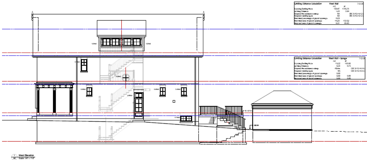
Proposed Side (West) Elevation – 29 St. Andrews Gardens Robert McCrea Architect, dated February 26, 2007
