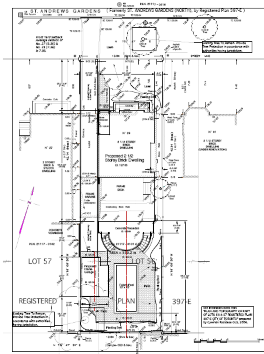
Proposed Site Plan – 29 St Andrews Gardens Robert McCrea Architect, dated February 26, 2007
