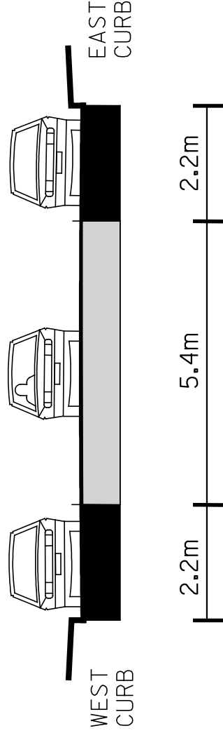
EXISTING CROSS SECTION A - A
