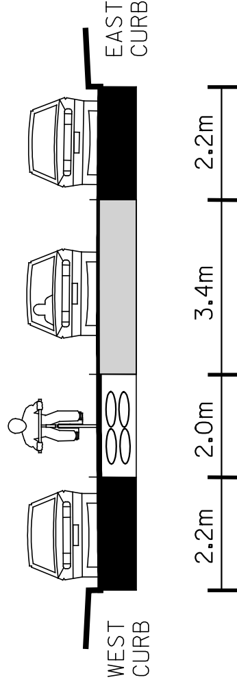
PROPOSED CROSS SECTION A - A
