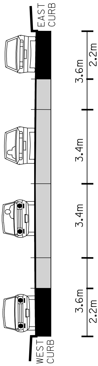
EXISTING CROSS SECTION A - A
