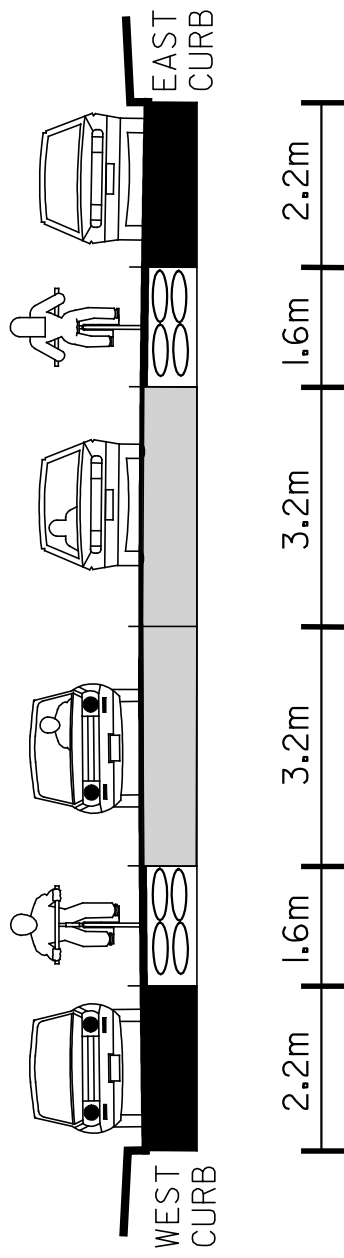
PROPOSED CROSS SECTION A - A
