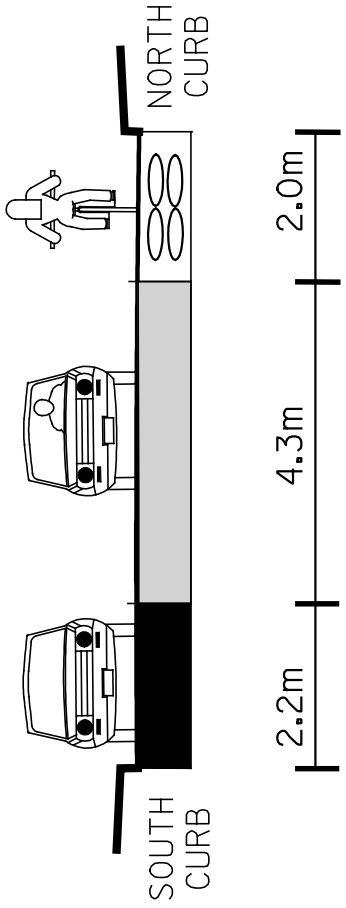
PROPOSED CROSS SECTION A - A
