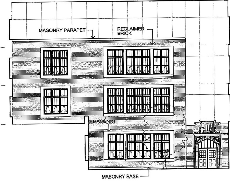
(B) WEST COURTYARD ELEVATION HERITAGE ARCH 1
