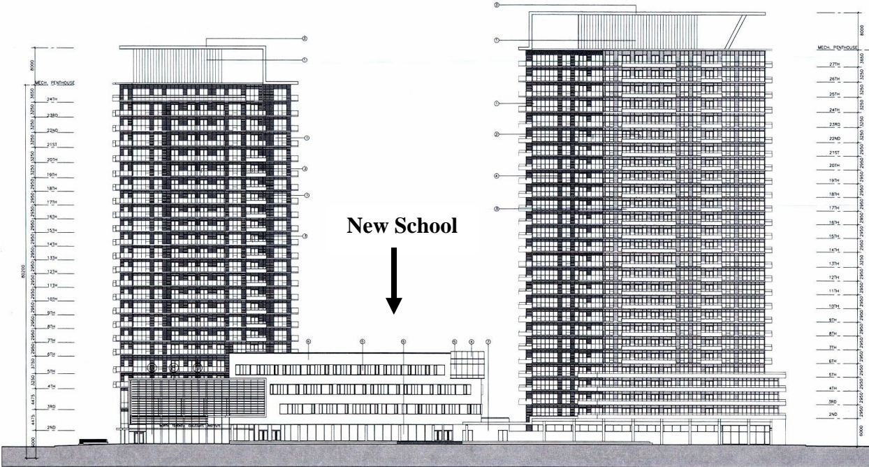
West Elevation
