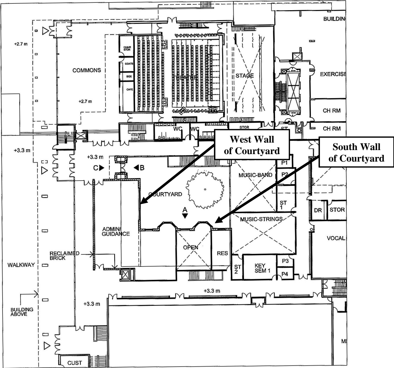
COURTYARD PLAN HERITAGE ELEMENTS
