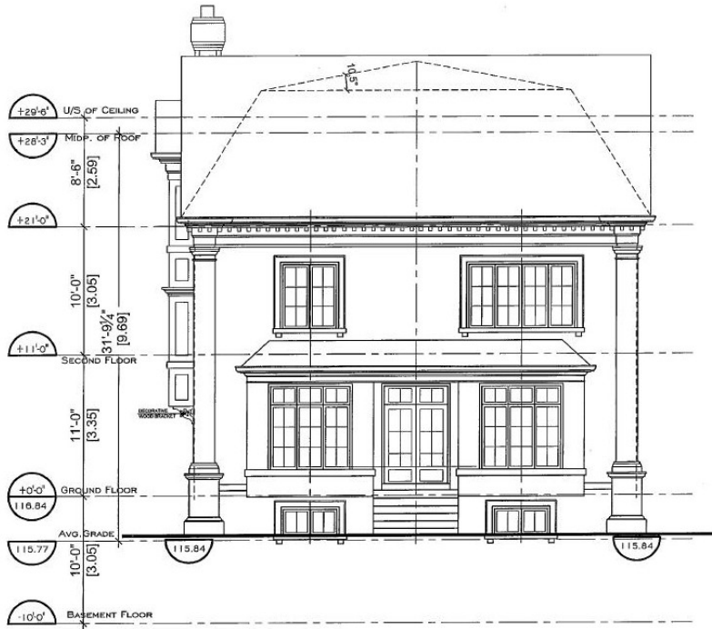
REAR ELEVATION
