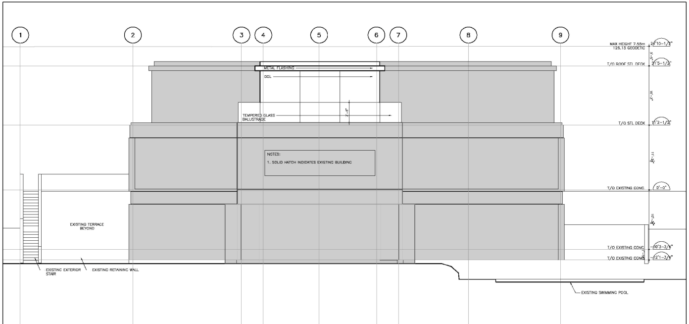
BUILDING ELEVATIONS 1 SOUTH A202
