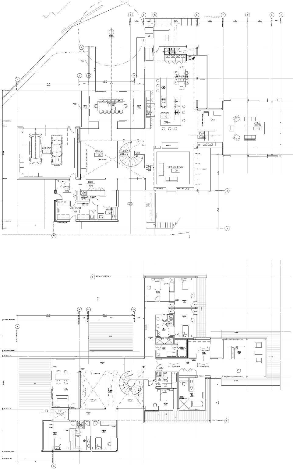
Top - Proposed main floor, Bottom – Proposed second floor
