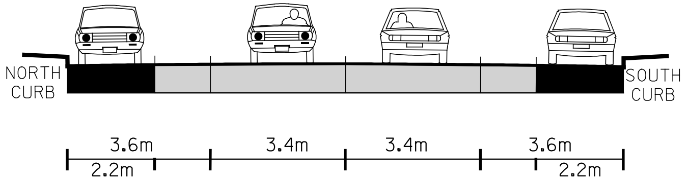
EXISTING CROSS SECTION B - B
