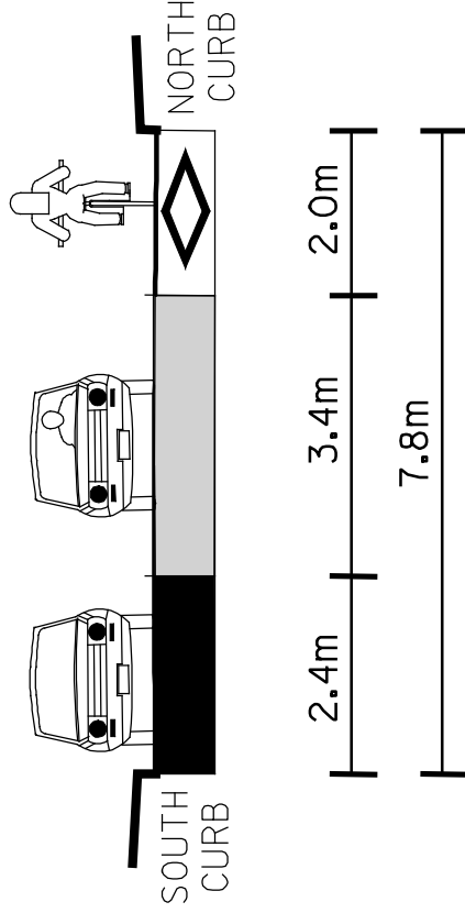
PROPOSED CROSS SECTION A - A
