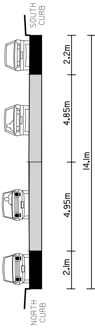
EXISTING CROSS SECTION A - A
