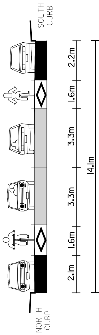
PROPOSED CROSS SECTION A - A
