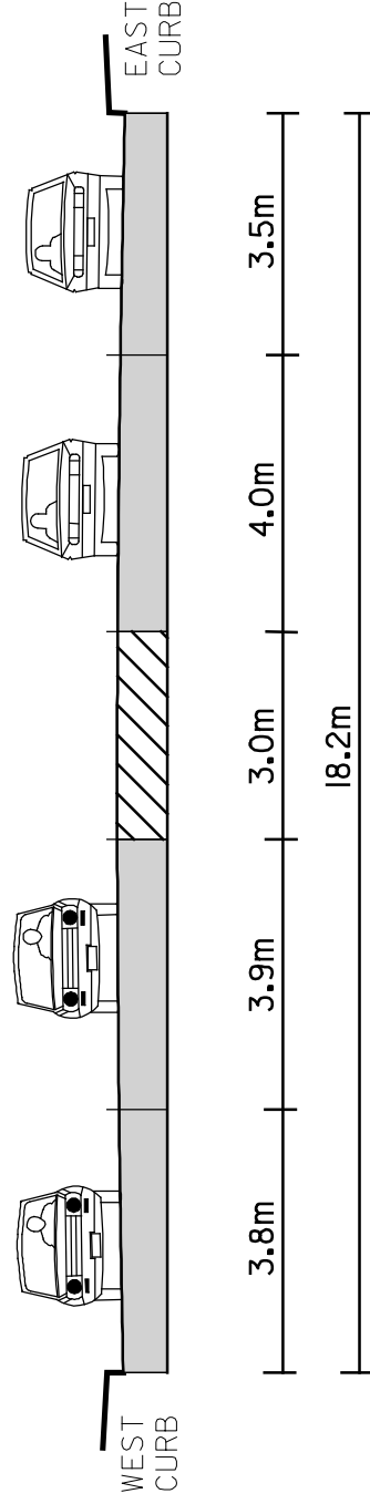
EXISTING CROSS SECTION A - A
