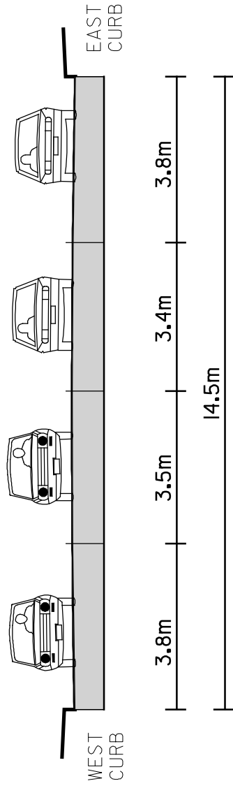
EXISTING CROSS SECTION A - A
