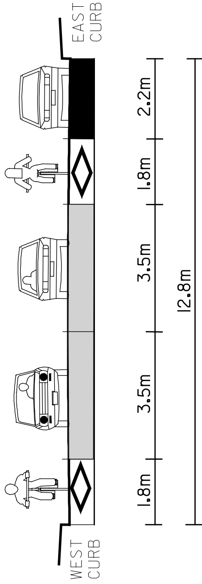
PROPOSED CROSS SECTION A - A
