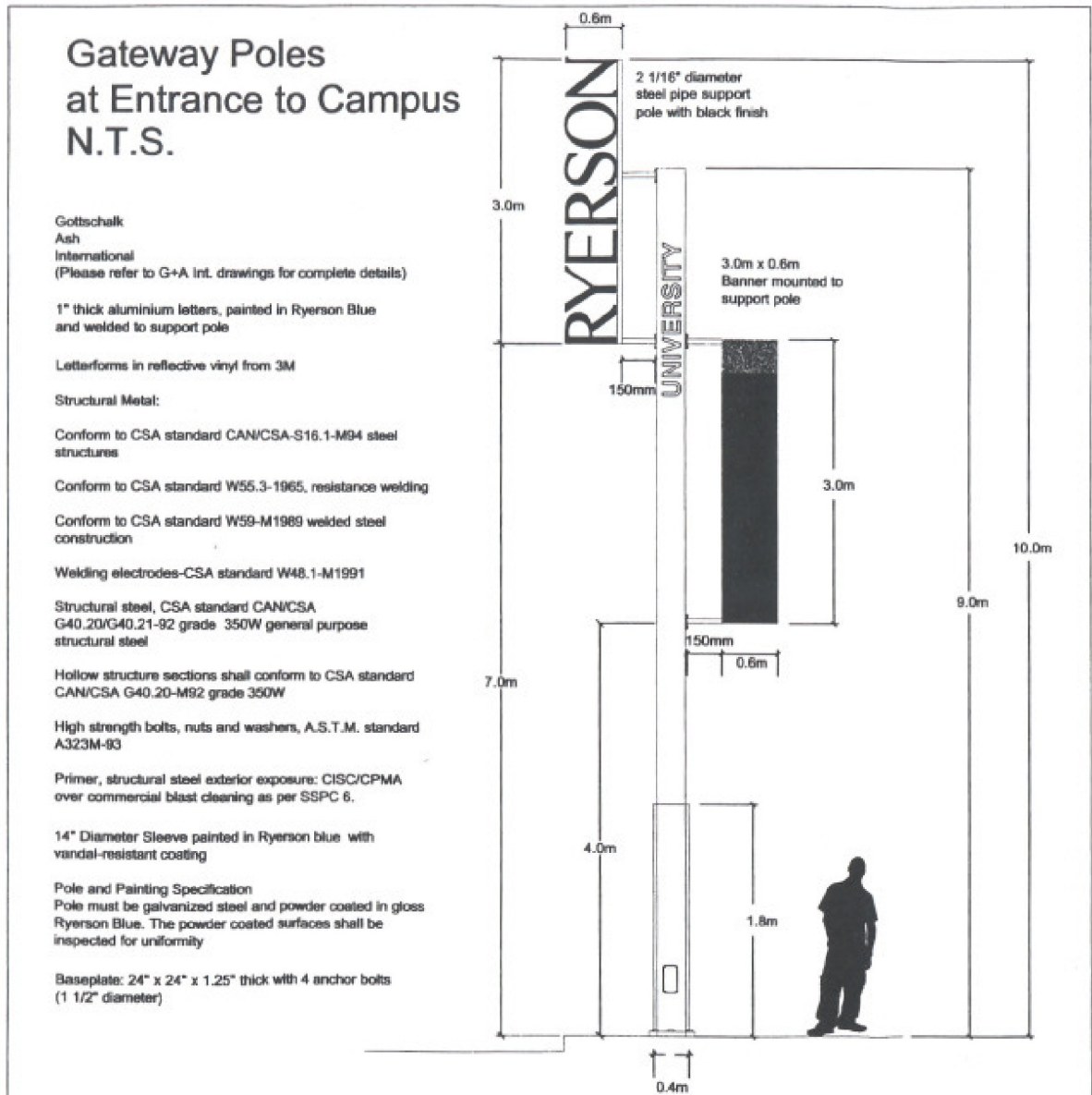
Conceptual drawing of proposed Ryerson gateway poles
