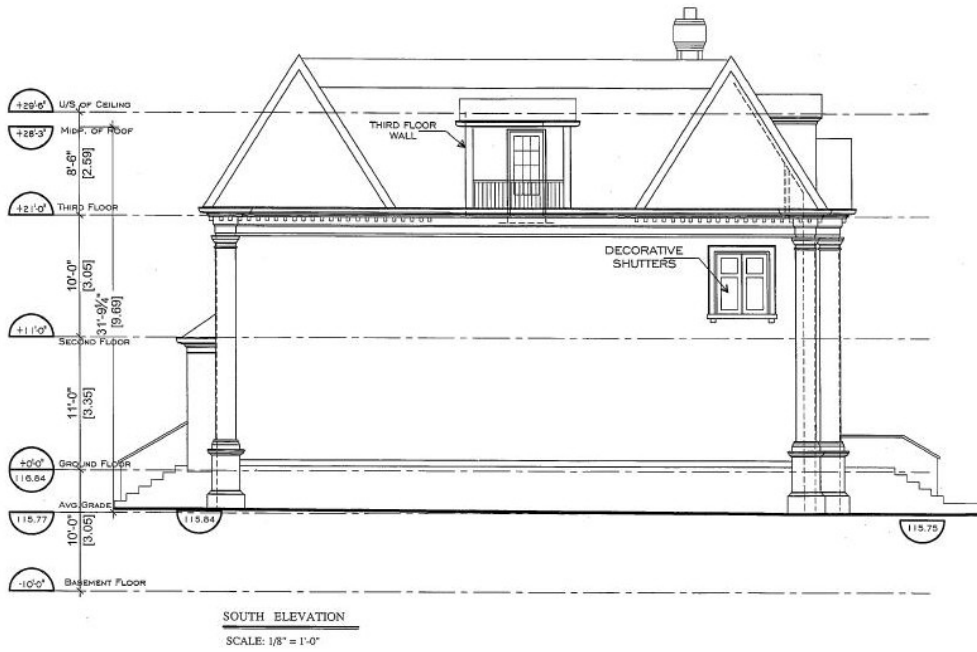
South elevation
