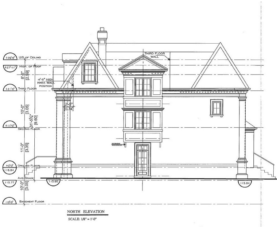
North elevation
