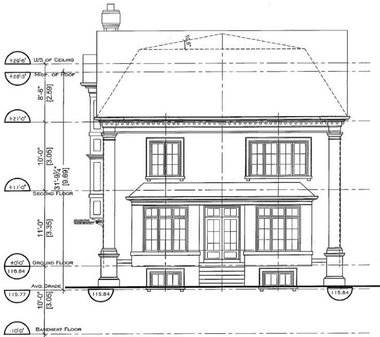
REAR ELEVATION
