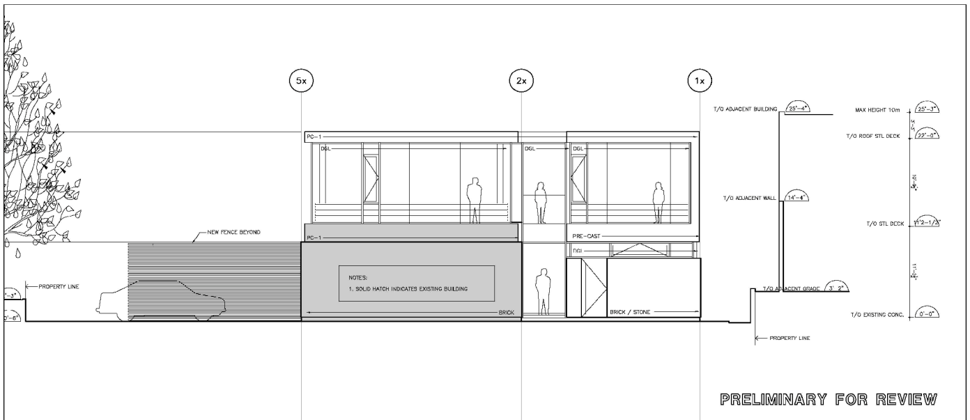
BUILDING ELEVATIONS 1 NORTH A202
