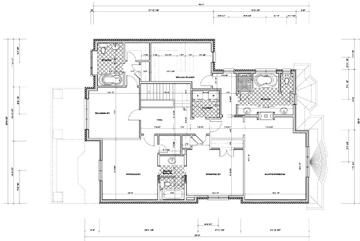
SECOND FLOOR PLAN SCALE: 1/4" = 1'-0" DATE: 11/15/11
