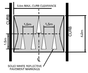
SPEED HUMP DETAIL
