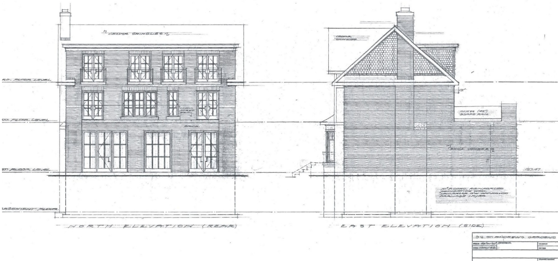
North Elevation
