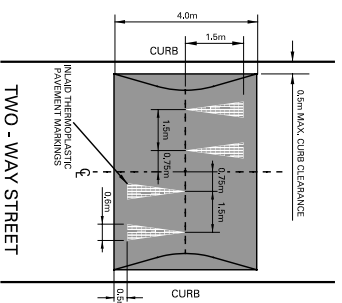
SPEED HUMP DETAIL
