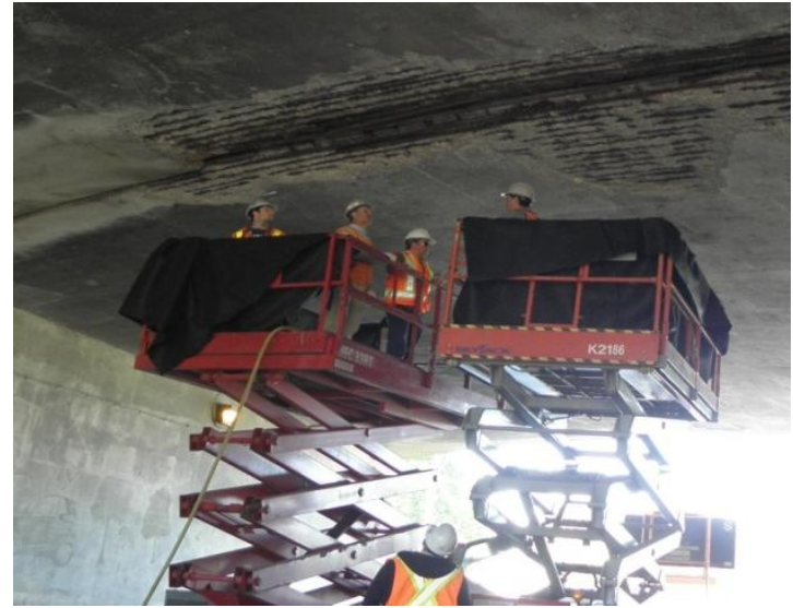
Visual Inspection and Controlled chipping
