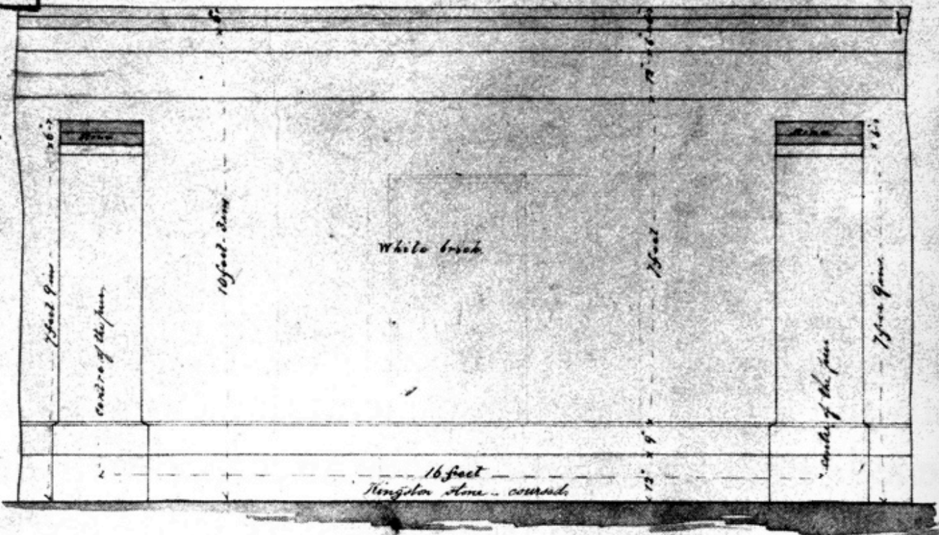
ELEVATION.
