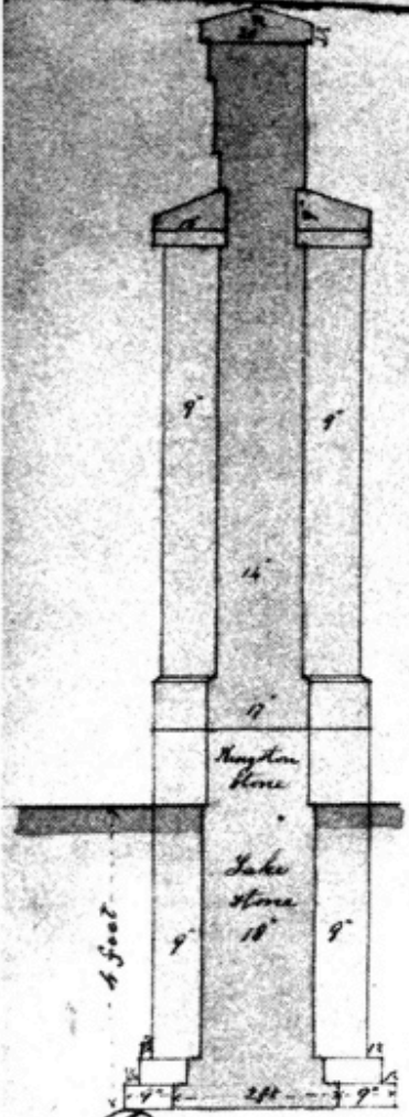
SECTION
