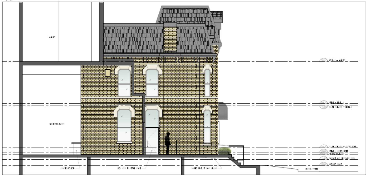
1 Partial Building Section Looking North
