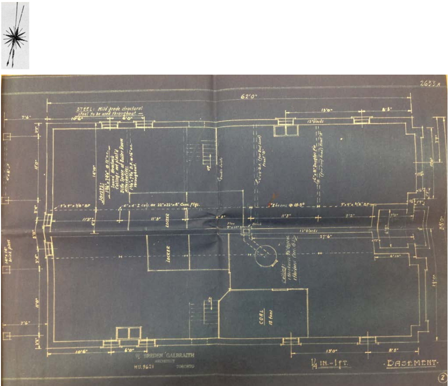
9. Basement Plan, as above, of a block, such as those at 1747, 1751 and 1755 Bayview Avenue which did not include garages (Building Records)
