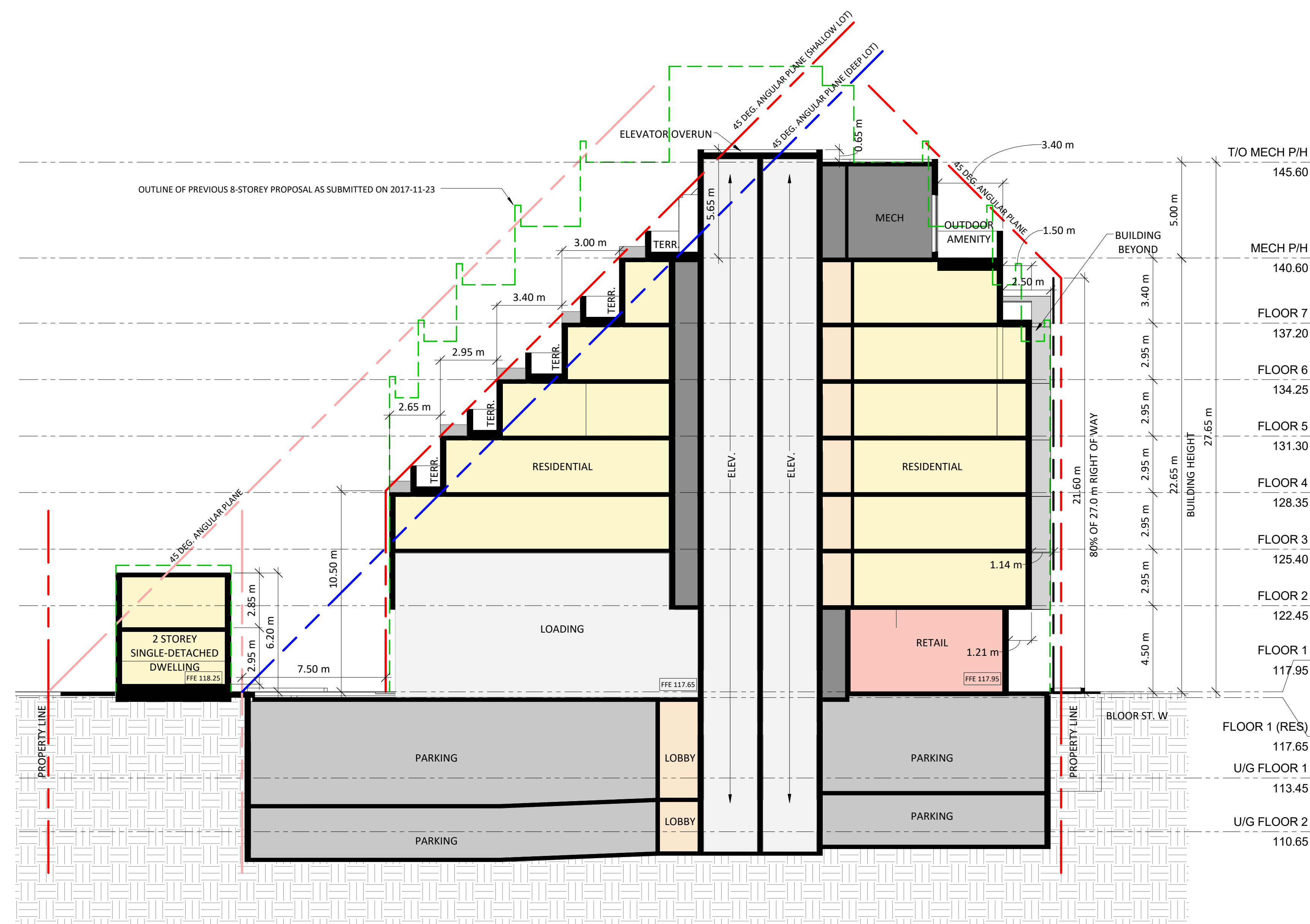
A SECTION A 1:150
