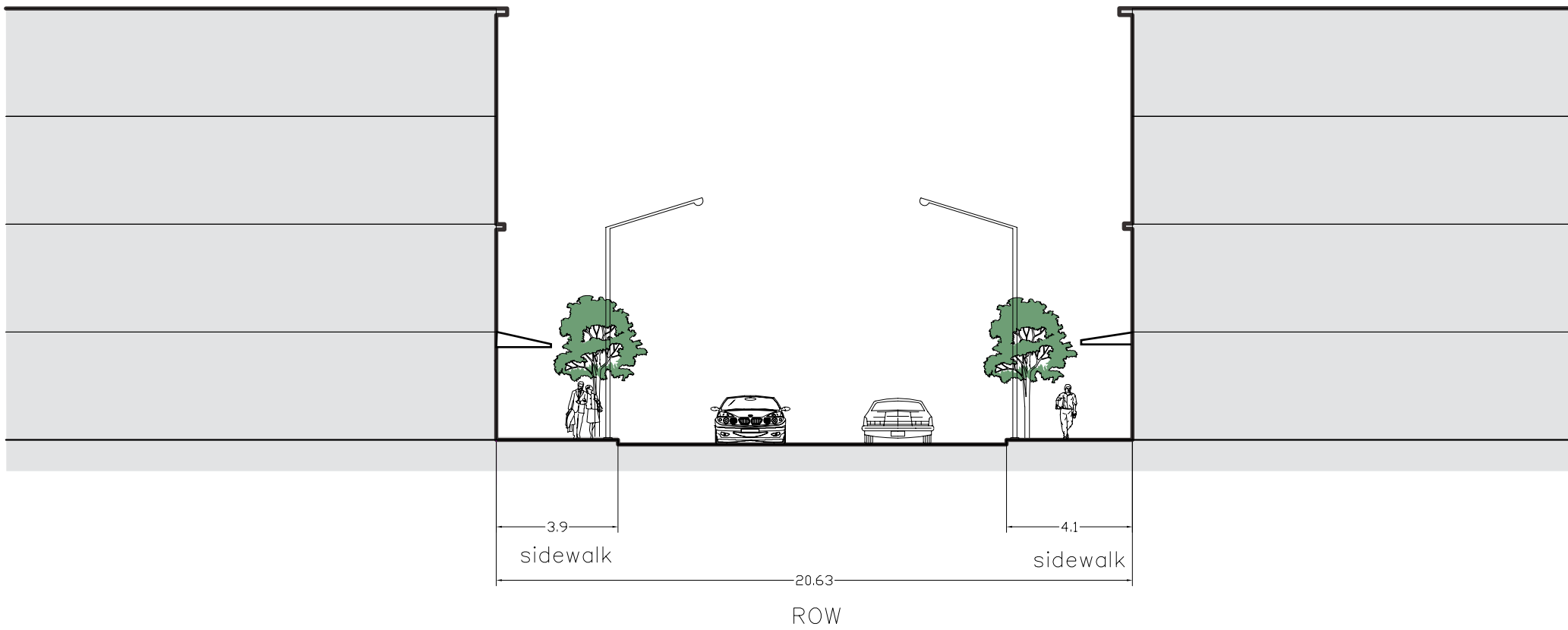
Section at DD
