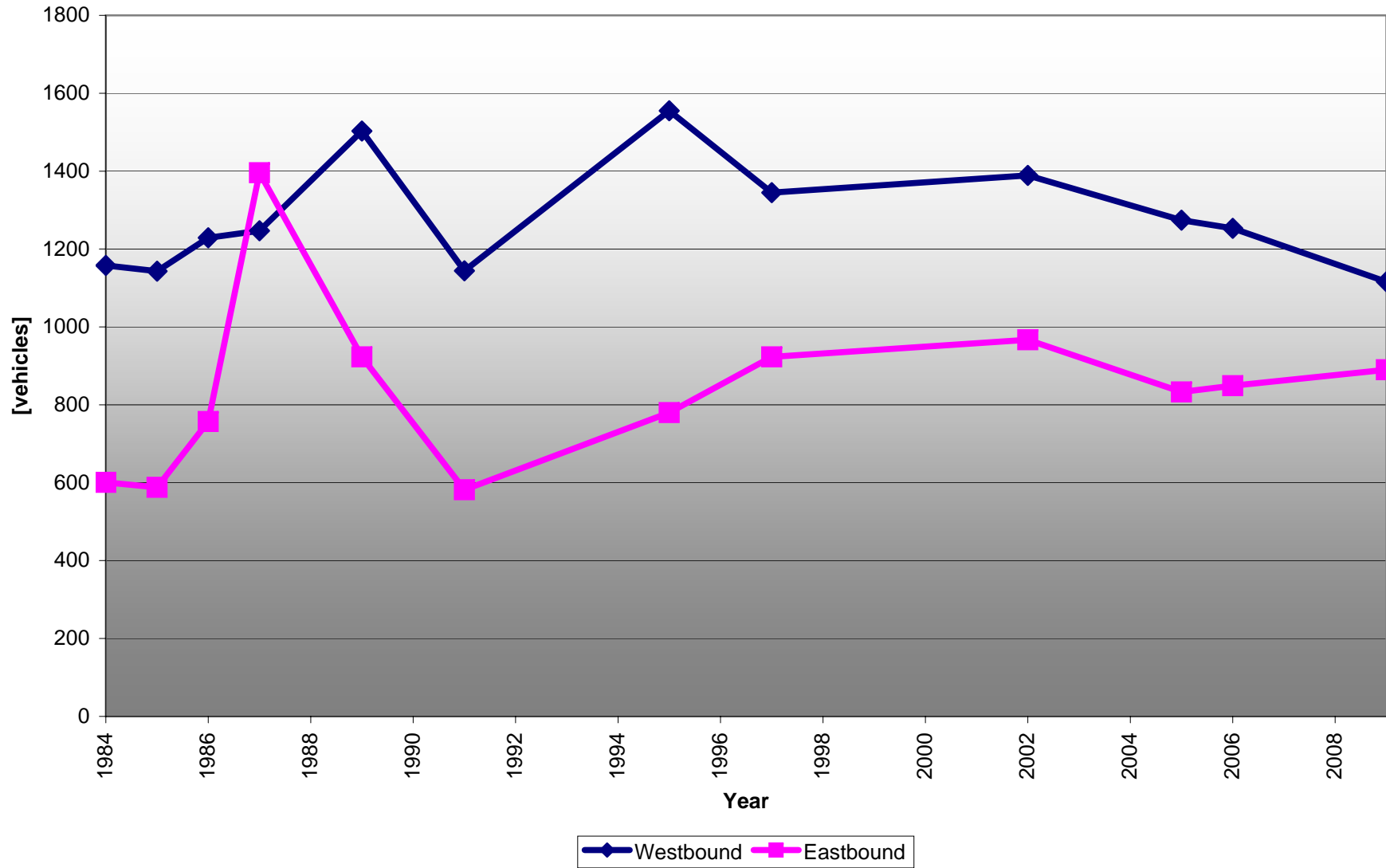
AM peak hour traffic growth on Finch Avenue, east of Warden Ave.
