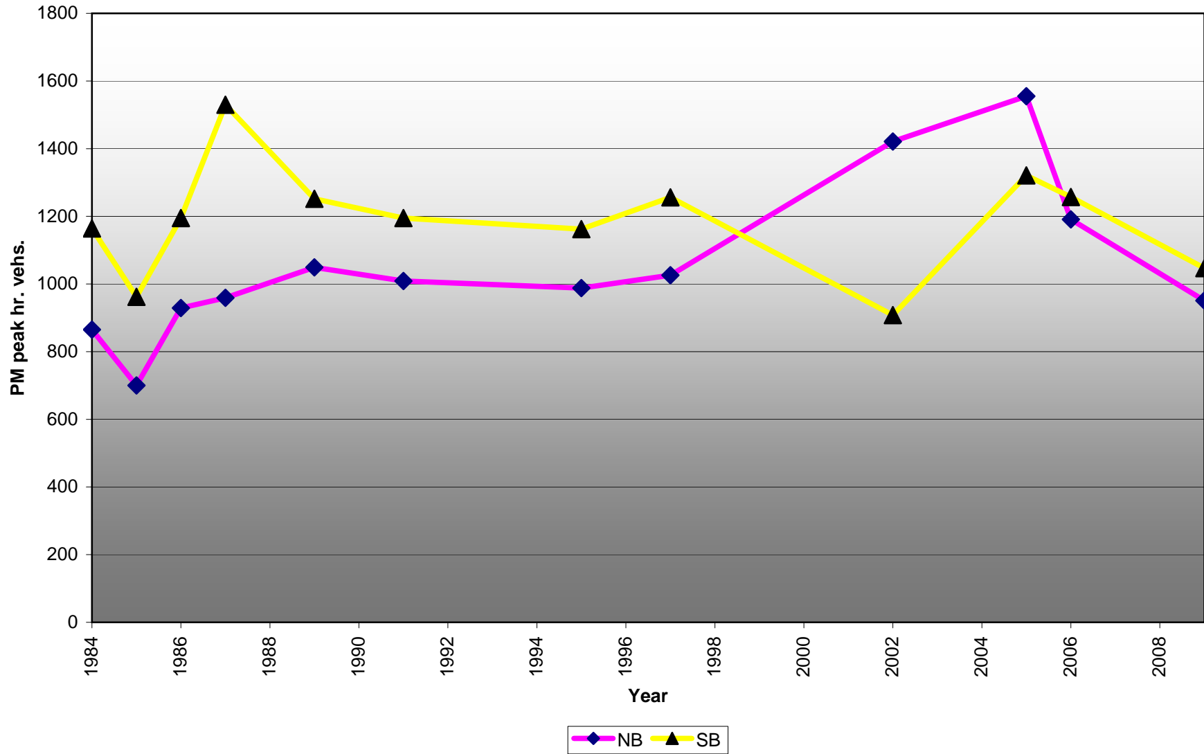
PM peak hour traffic growth on Warden Ave. N of Finch Ave.
