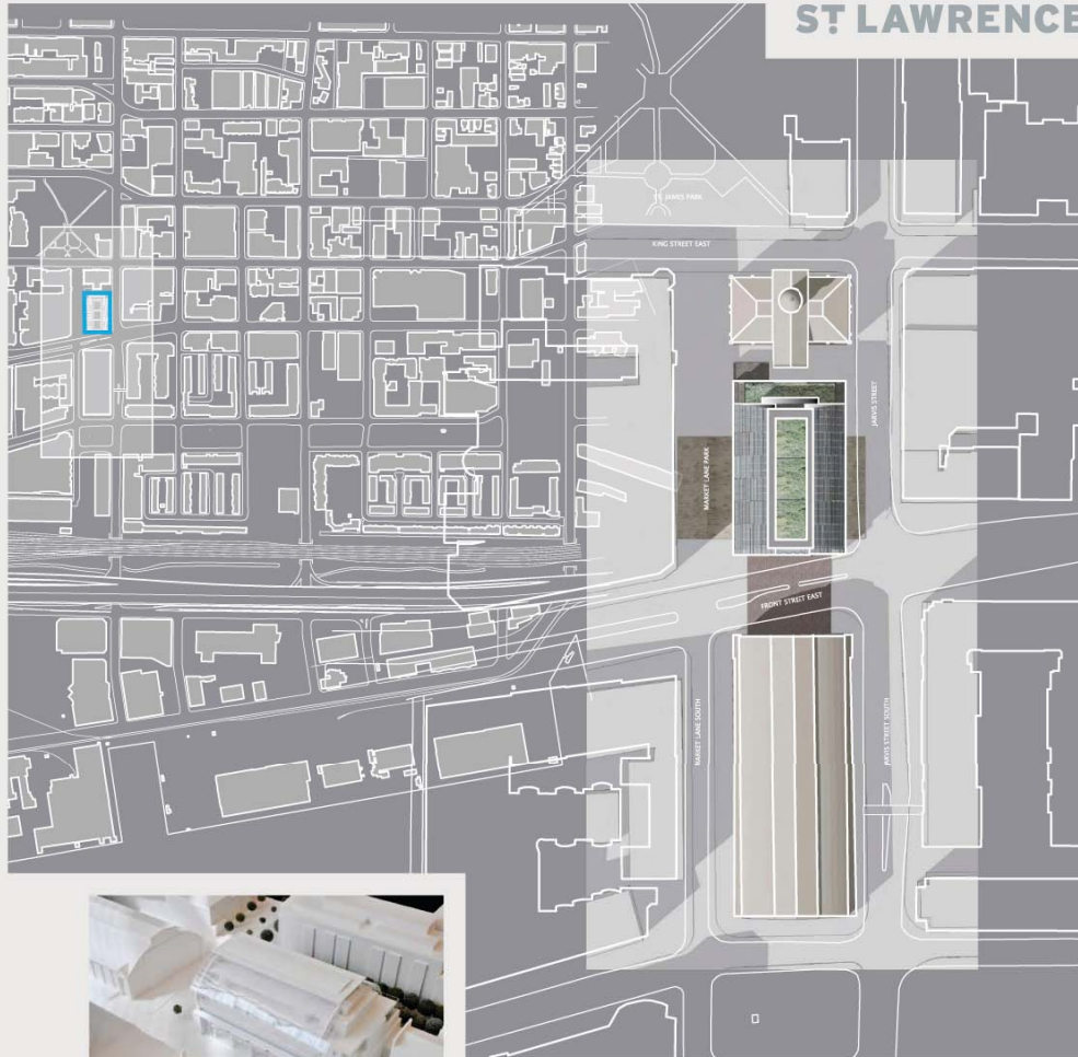
SPRING/FALL EQUINOX
