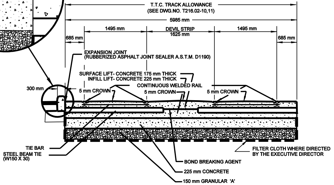
AT GRADE TYPICAL CROSS SECTION 'B'
