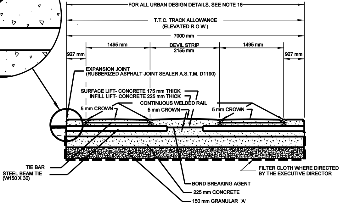
ELEVATED R.O.W. TYPICAL CROSS SECTION 'A'
