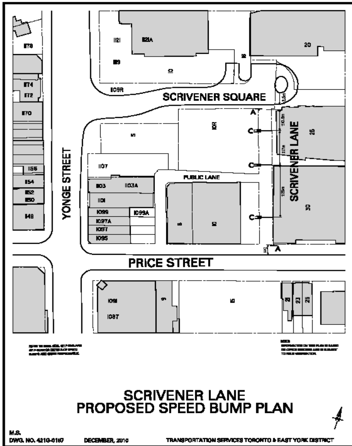
Drawing No. 421G-0187
