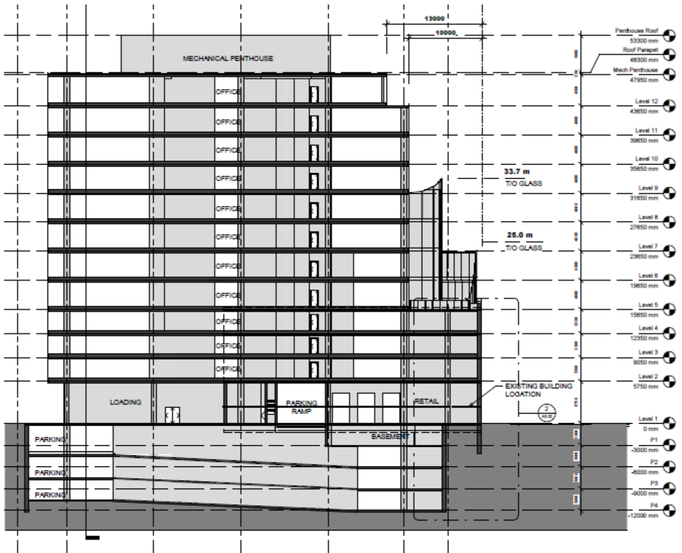
1 Section - South / North 1 : 200
