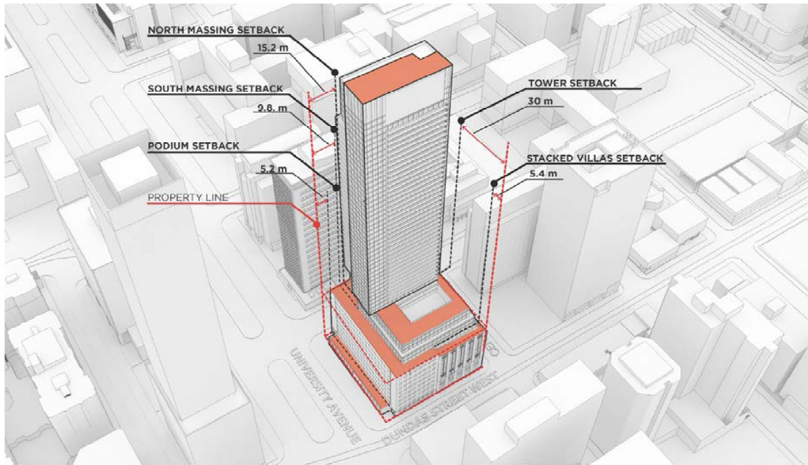
Rendering of Proposed Tower Stepbacks from Heritage Facades
