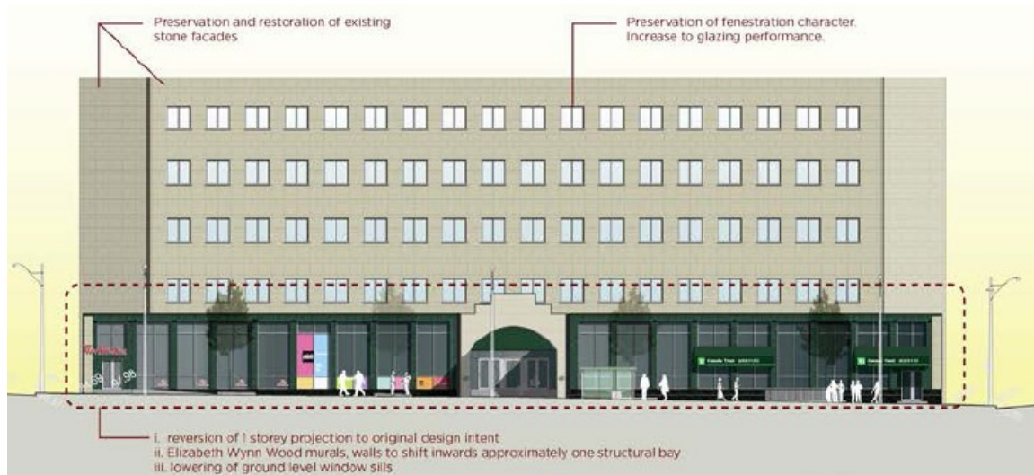
Existing West Elevation (University Avenue)
