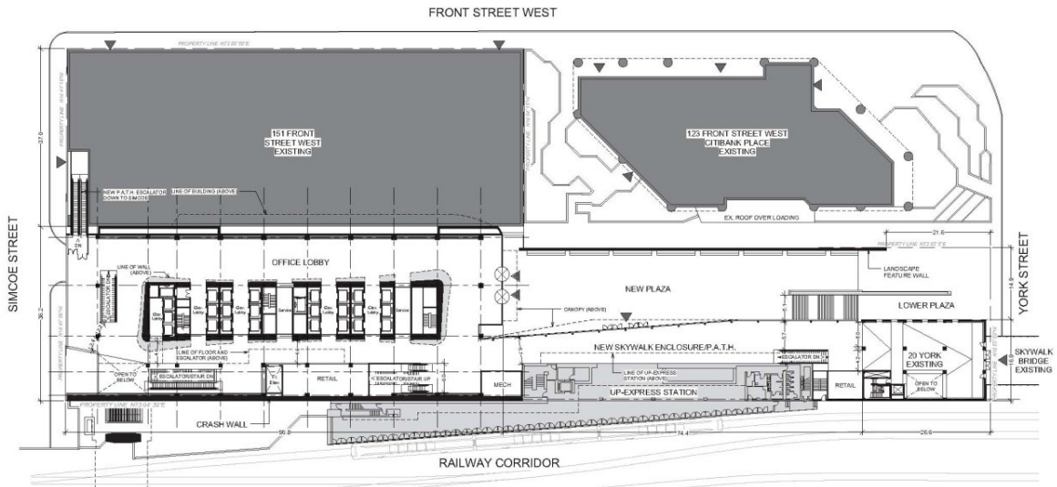
Plaza Level Plan
