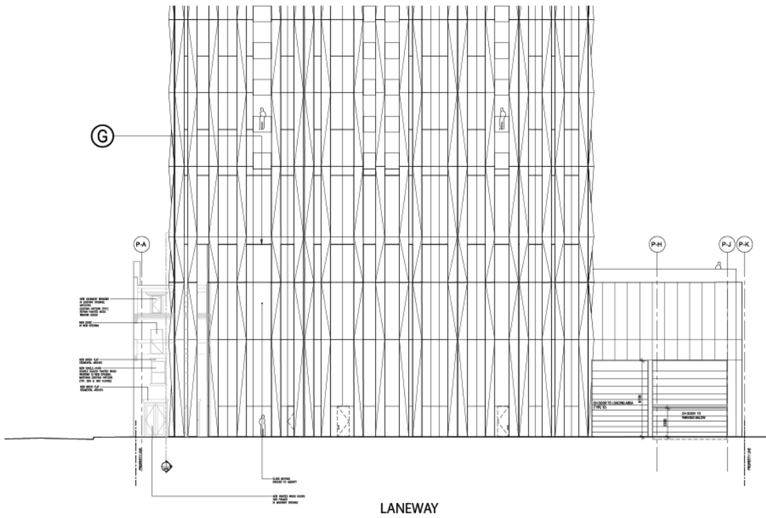
Laneway Elevation (West Elevation)
