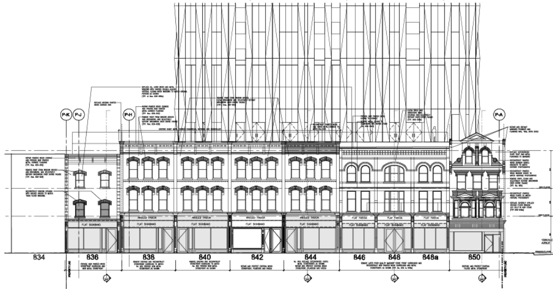
Yonge Street Podium Elevation (East Elevation)
