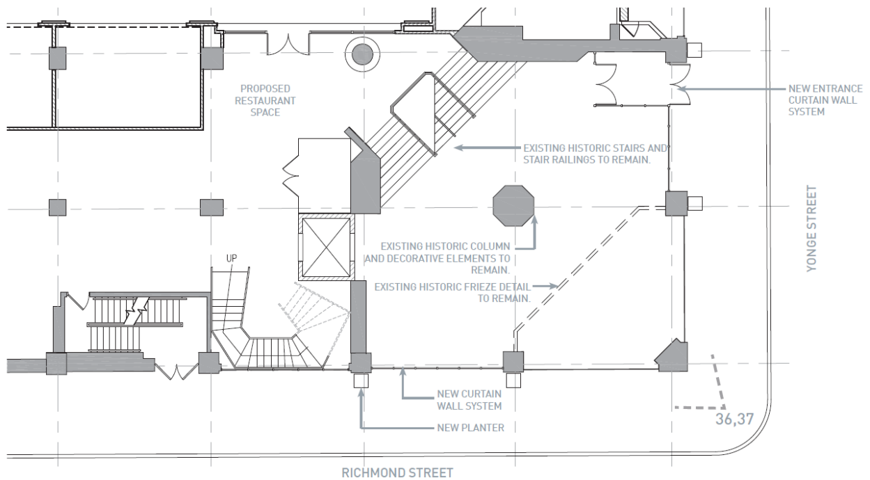
Richmond and Yonge Street Lobby – Proposed
