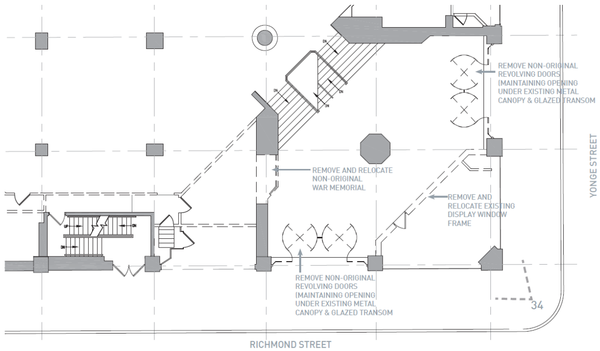
Richmond and Yonge Street Lobby – Demolition Plan
