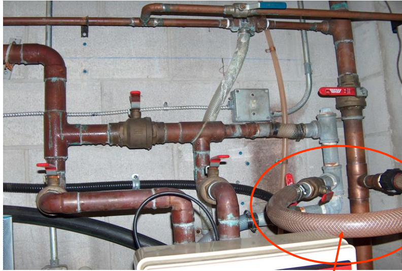
Booster Pump 80 PSI City Pressure 65 PSI
