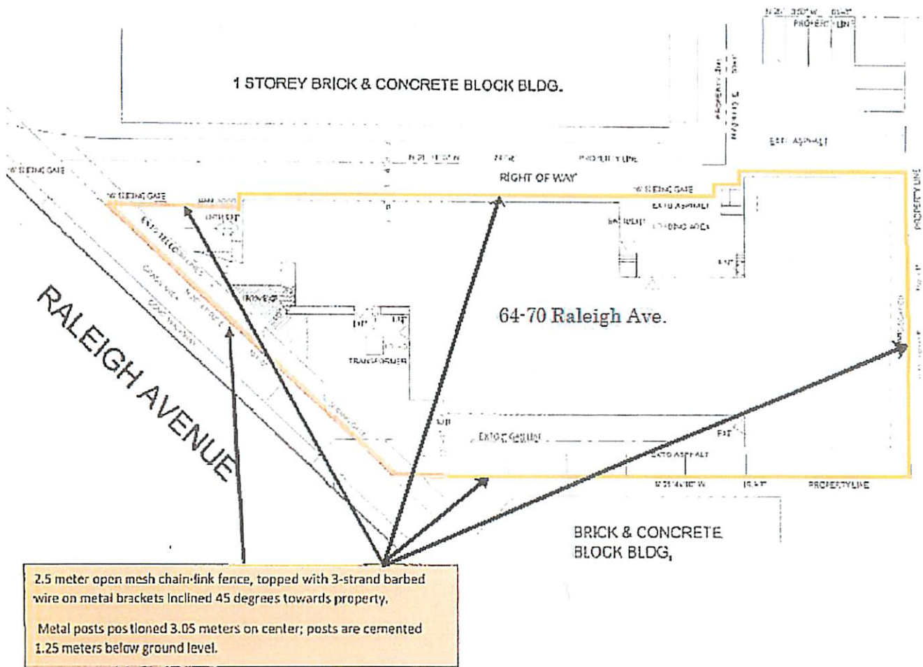
Appendix 2 – Proposed Fence Location Plan View.
