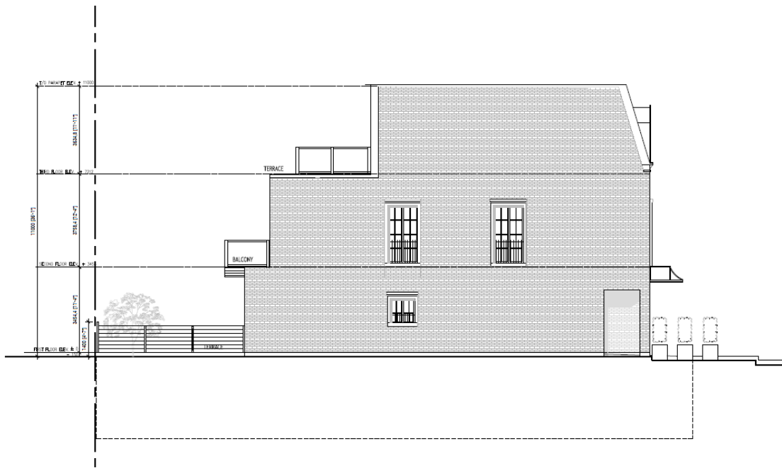
West Elevation
