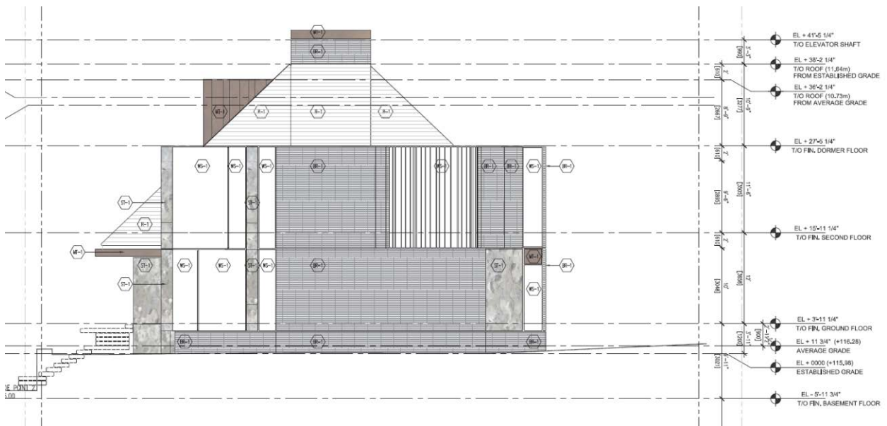
South Elevation
