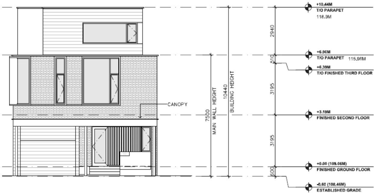
East (main) elevation
