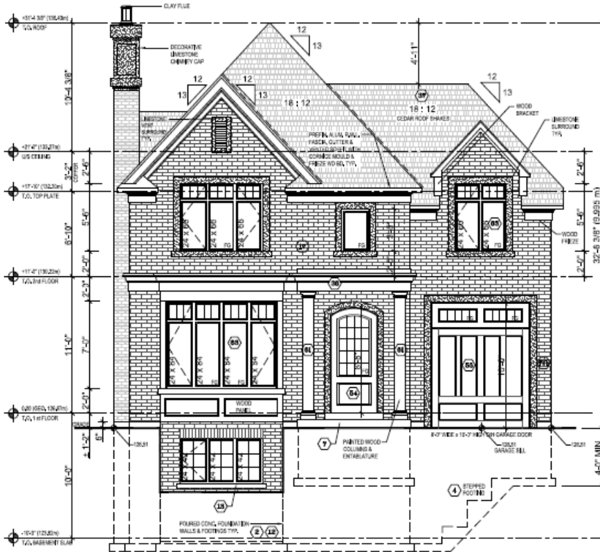
North (Primary) Elevation
