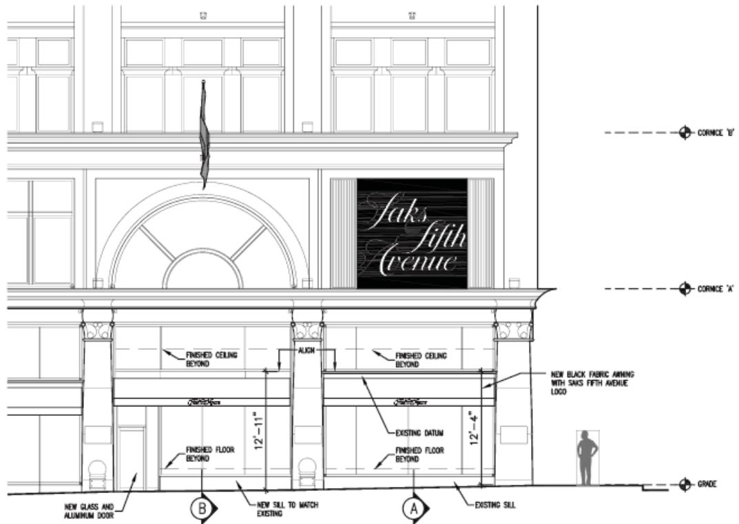
2 ELEVATION at YONGE STREET SCALE: 1/8" = 1'-0"
